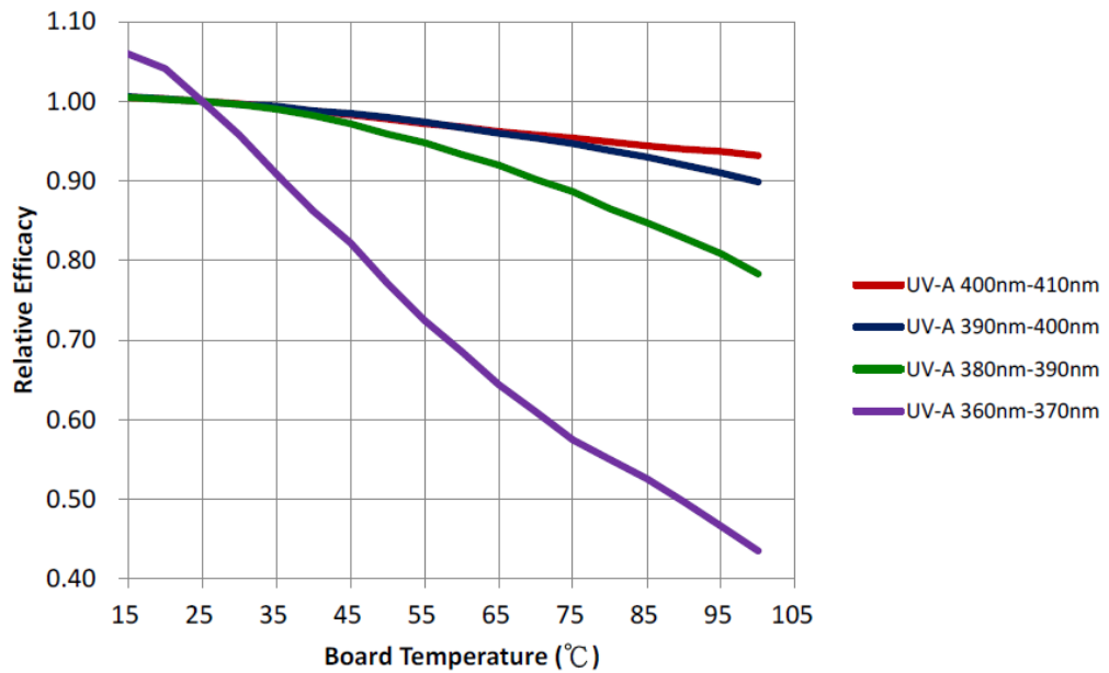
Relative Luminous Intensity vs Ambient Temperature
