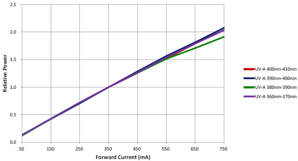
Forward current vs. Relative luminous intensity
