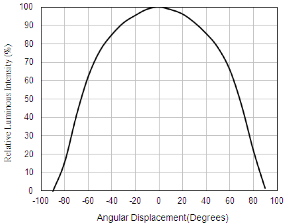
Typical Representative Spatial Radiation Pattern
