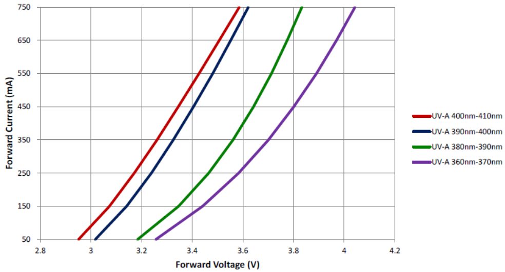
Forward Voltage vs. Forward Current
