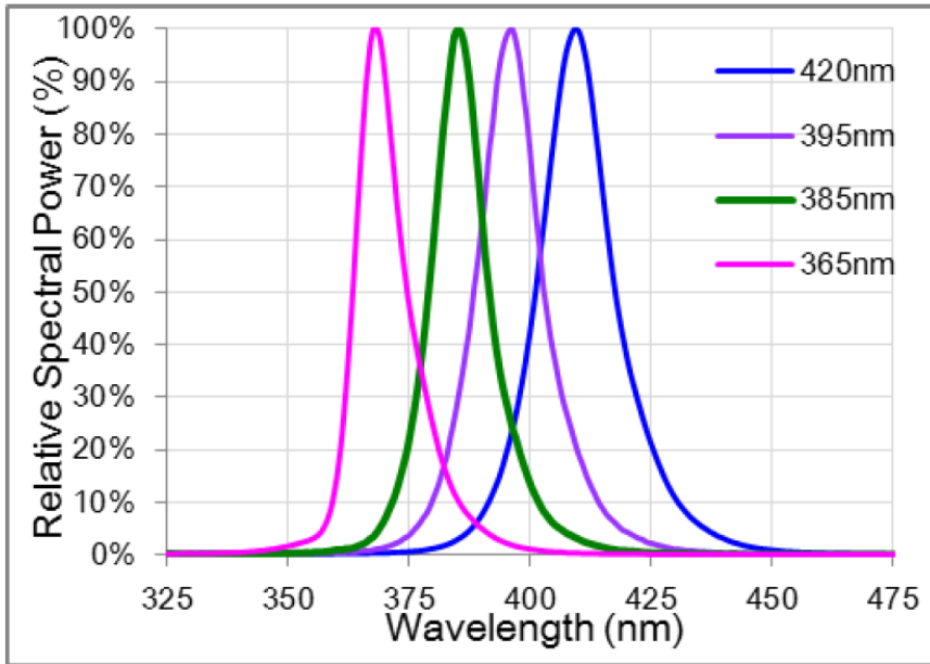
Spectrum Distribution
