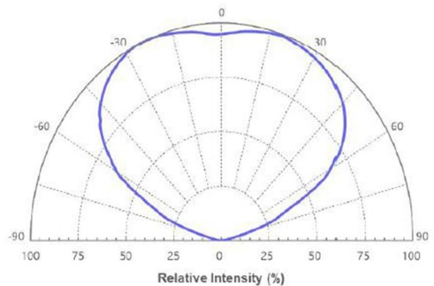
Typical Representative Spatial Radiation Pattern
