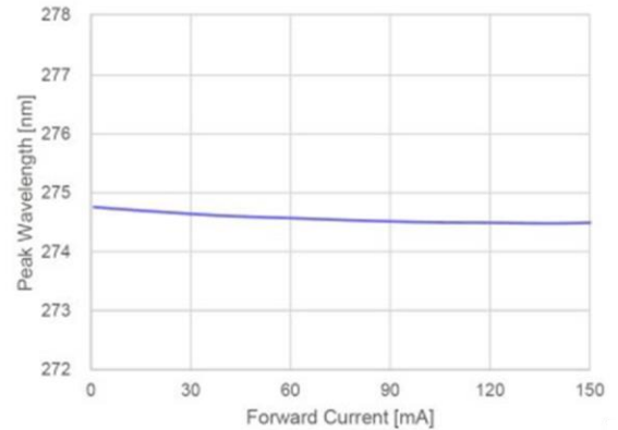
Forward Current vs. Peak Wavelength
