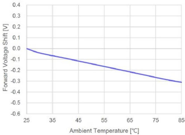
Forward Voltage Shift vs. Ambient Temperature
